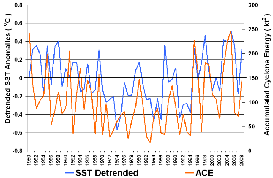
Figure 2: Tropical North Atlantic Sea Surface Temperature Anomalies (Aug.-Sept.) and North Atlantic Accumulated Cyclone Energy (1950-2008)
